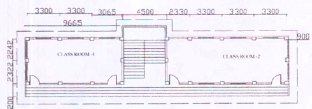
GROUND FLOOR PLAN NIFT B. ED COLLEGE
