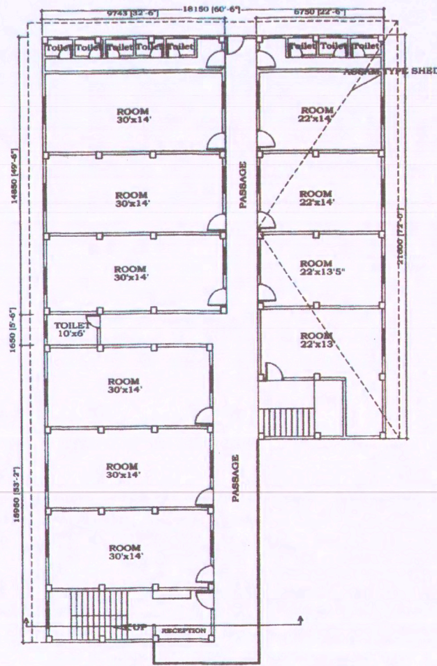
FIRST & SECOND FLOOR scale :- 1:100
