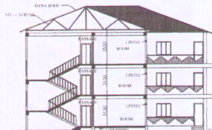
SECTIONAL ELEVATION AT AA [BLOCK A]
