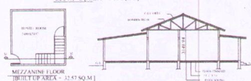
MEZZANINE FLOOR [BUILT UP AREA = 32.57 SQ.M] SECTION AT BB BLOCK - B NATIONAL INSTITUTE FOR TEACHER EDUCATION.
