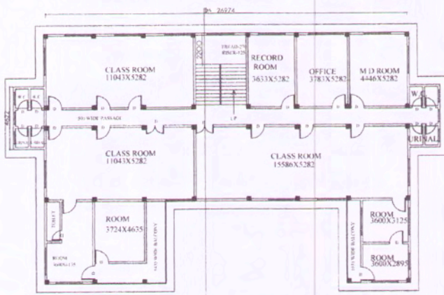
FIRST FLOOR PLAN [BUILT UP AREA= 446.31 SQ. M] BLOCK - A NATIONAL INSTITUTE FOR TEACHER EDUCATION.
