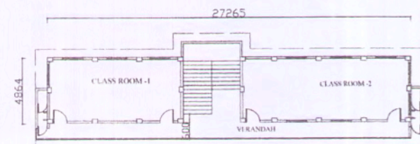
SECOND FLOOR PLAN NIFT B. ED COLLEGE
