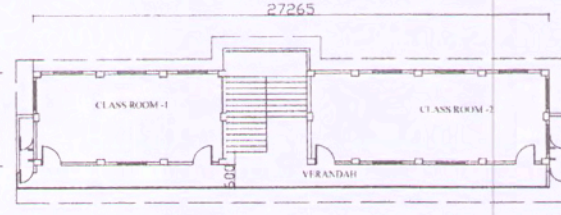
FIRST FLOOR PLAN NIFT B. ED COLLEGE
