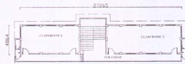
THIRD FLOOR PLAN NIFT B. ED COLLEGE
