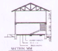
SECTION MM SECTION AT MEZZANINE FLOOR
