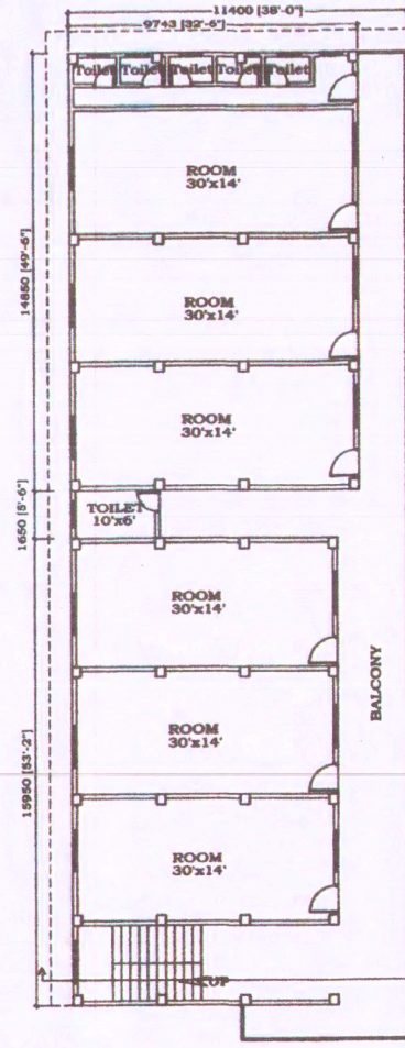
THIRD FLOOR scale :- 1:100
