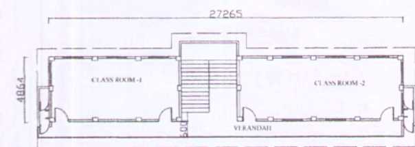
FOURTH FLOOR PLAN NIFT B. ED COLLEGE
